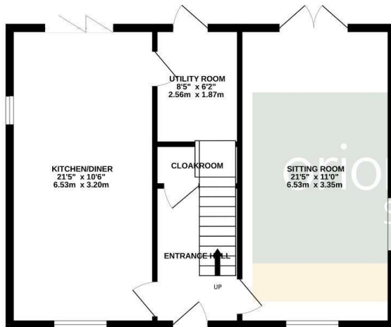
GROUND FLOOR 592 sq.ft. (55.0 sq.m.) approx.
