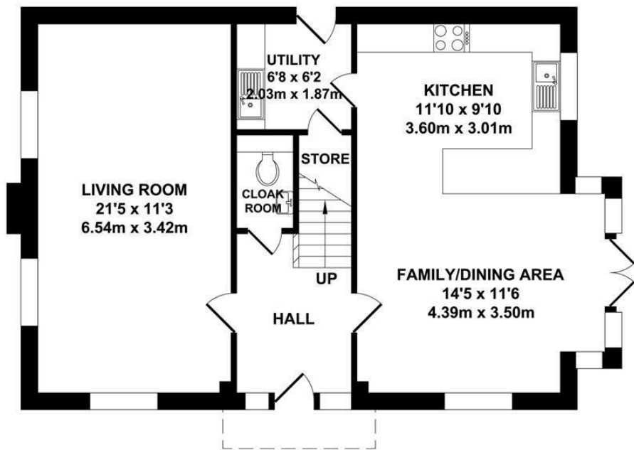
GROUND FLOOR APPROX. FLOOR AREA 675 SQ.FT. (62.71 SQ.M.)
