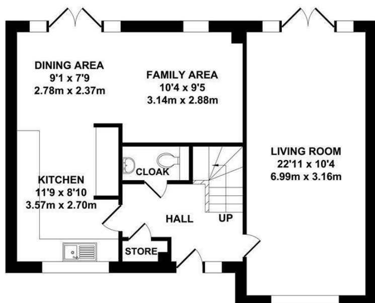
GROUND FLOOR APPROX. FLOOR AREA 639 SQ.FT. (59.33 SQ.M.)
