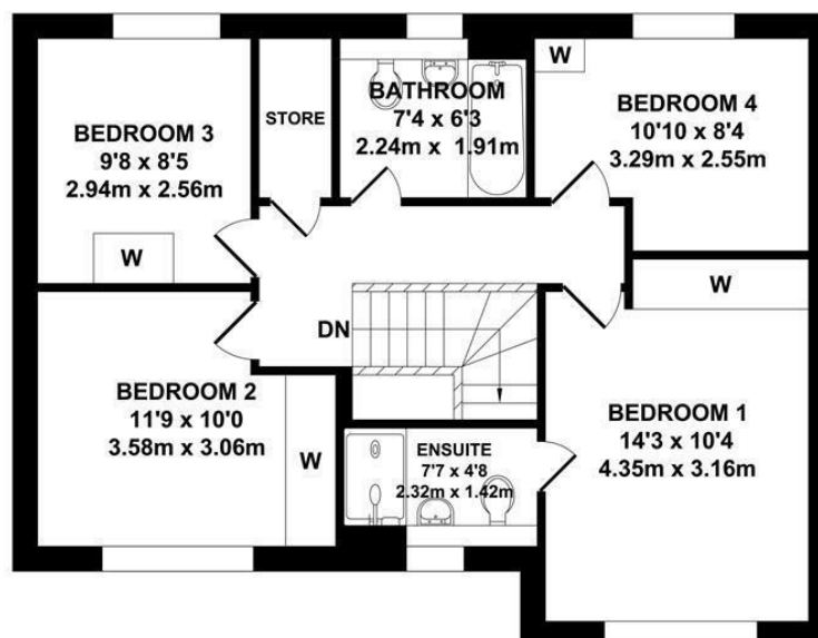
FIRST FLOOR APPROX. FLOOR AREA 632 SQ.FT. ( 58.67 SQ.M.)
