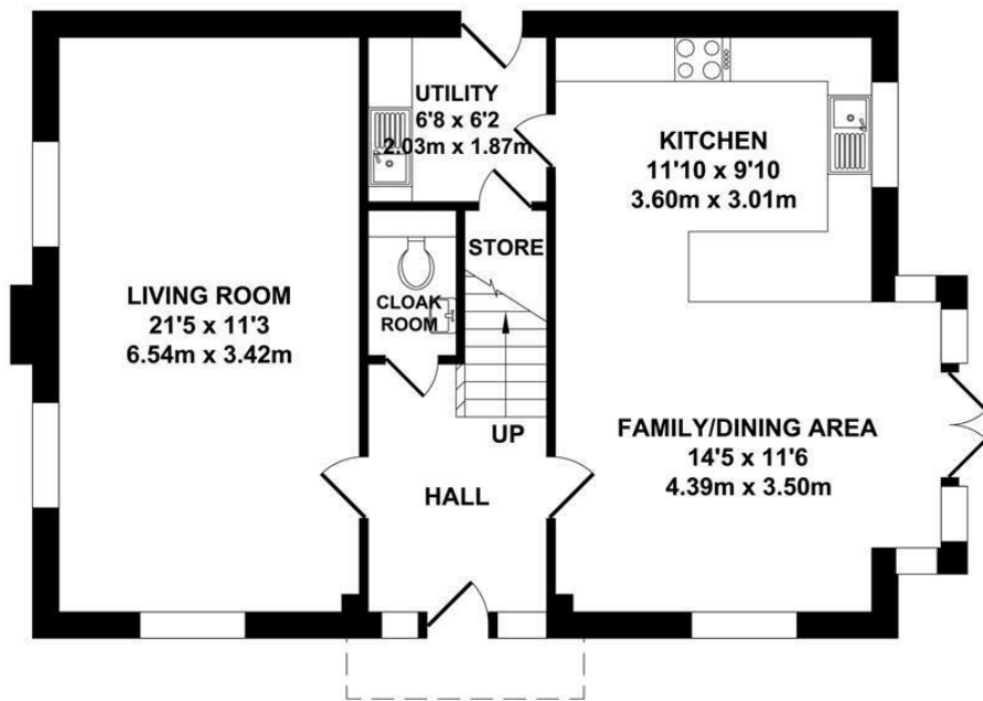
GROUND FLOOR APPROX. FLOOR AREA 675 SQ.FT. (62.71 SQ.M.)
