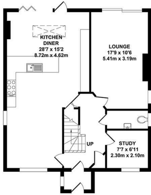
GROUND FLOOR APPROX. FLOOR AREA 762 SQ.FT. (70.80 SQ.M.)
