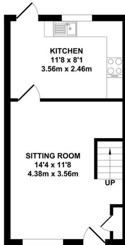
GROUND FLOOR APPROX. FLOOR AREA 266 SQ. FT. (24.71 SQ. M)
