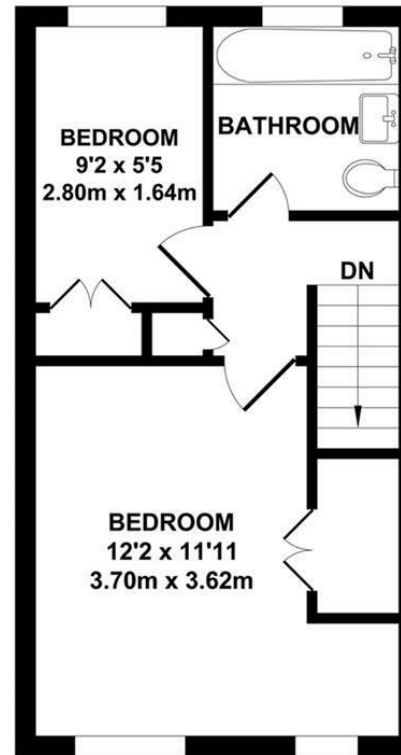
FIRST FLOOR APPROX. FLOOR AREA 266 SQ. FT. (24.71 SQ. M)
