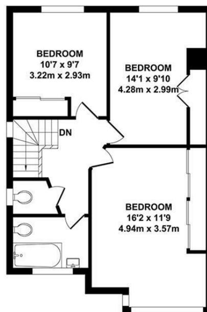
FIRST FLOOR APPROX. FLOOR AREA 552 SQ.FT. (51.25 SQ.M.)
