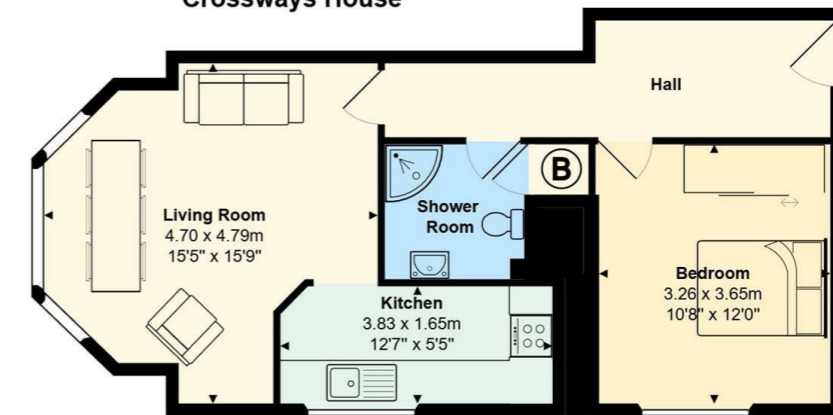
Crossways House
