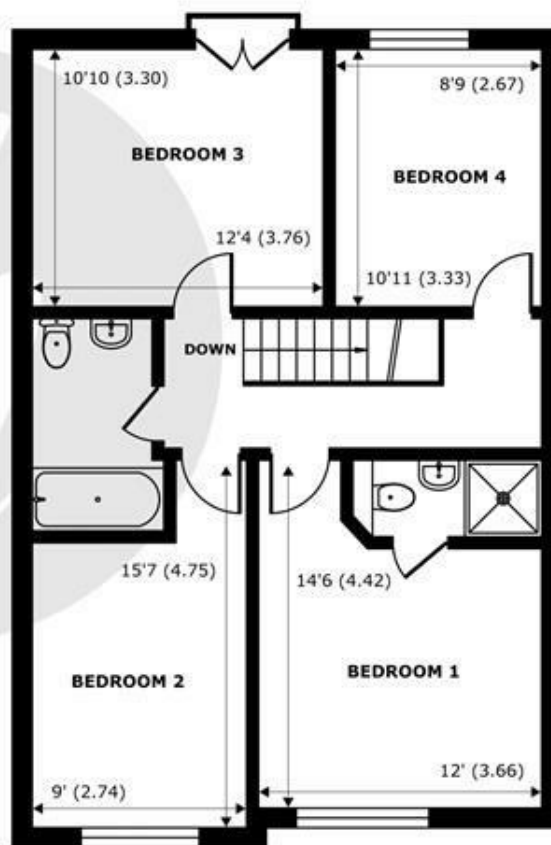
FIRST FLOOR abt 796 SQFT (74 SQMT)
