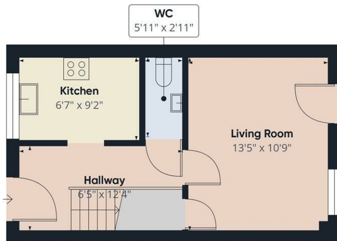
Floor 0
