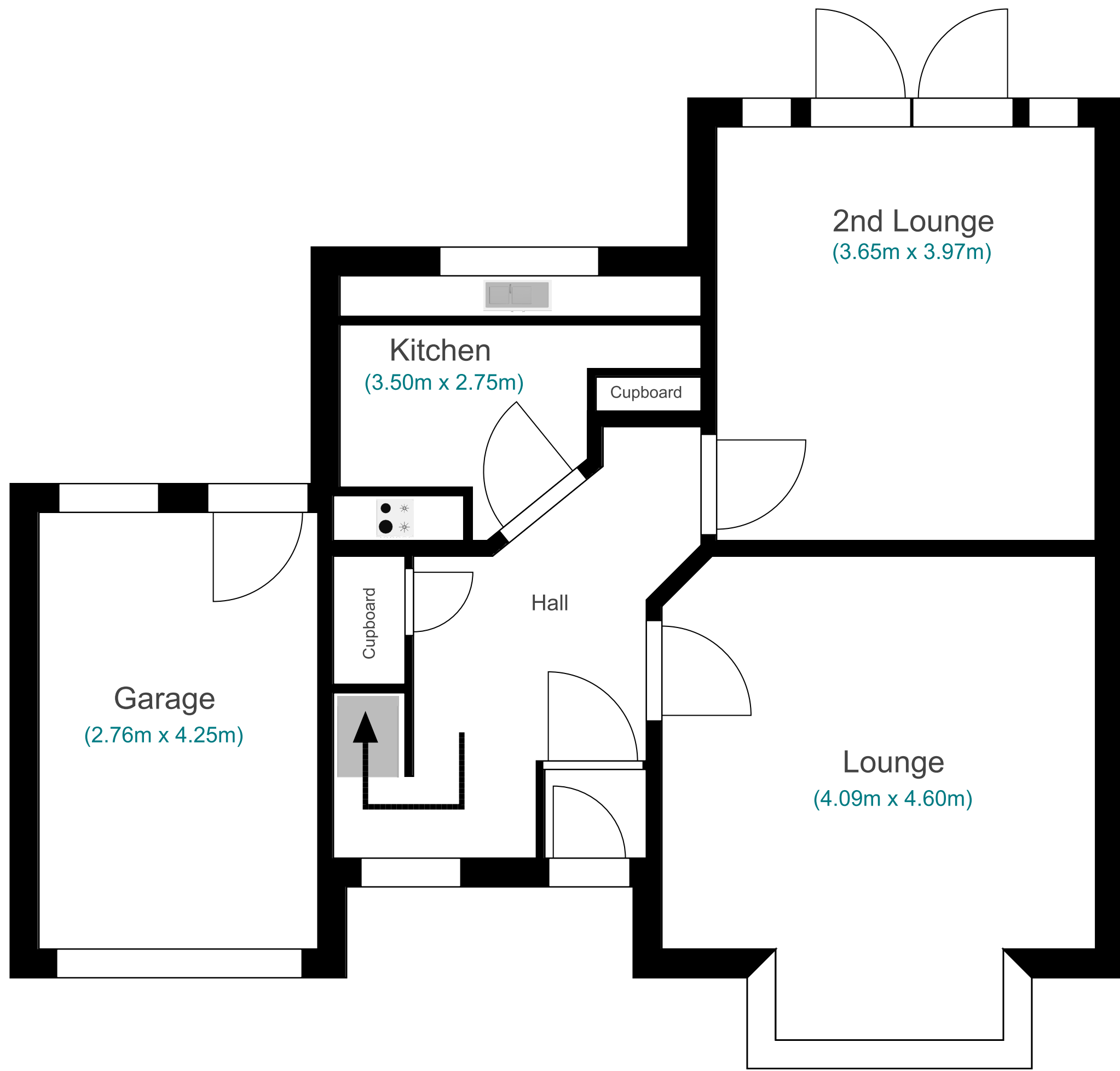
Ground Floor
