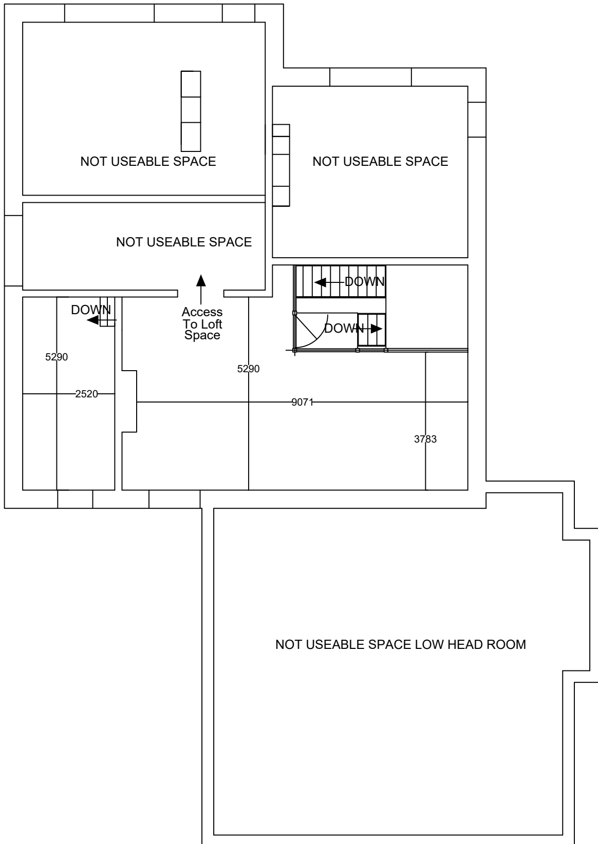
SECOND FLOOR
