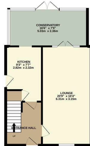
GROUND FLOOR 500 sq.ft. (46.4 sq.m.) approx.
