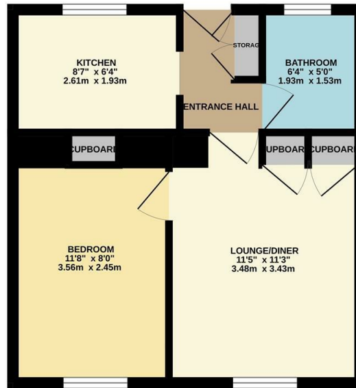
FIRST FLOOR 331 sq.ft. (30.8 sq.m.) approx.
