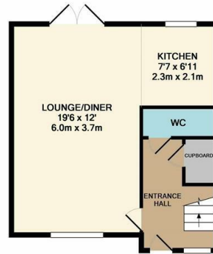
GROUND FLOOR APPROX. FLOOR AREA 381 SQ.FT. (35.4 SQ.M.)
