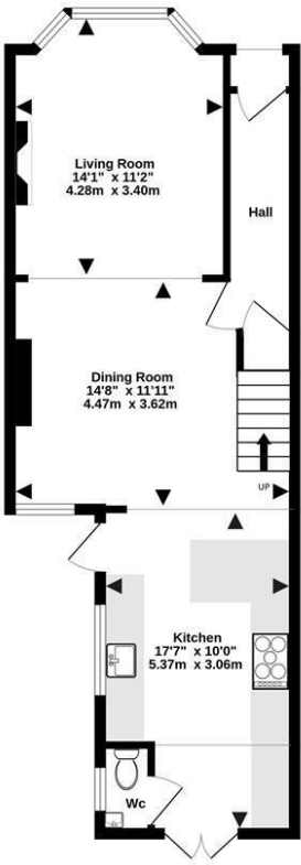
GROUND FLOOR 521 sq.ft. (48.4 sq.m.) approx.
