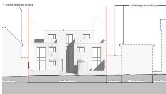
NORTH ELEVATION - FRONT
