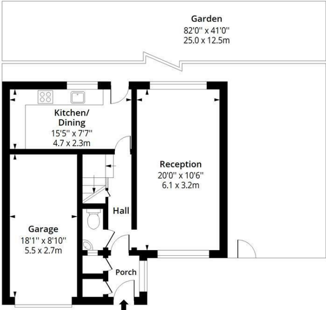
Ground Floor Floor Area 477 Sq Ft - 44.31 Sq M
