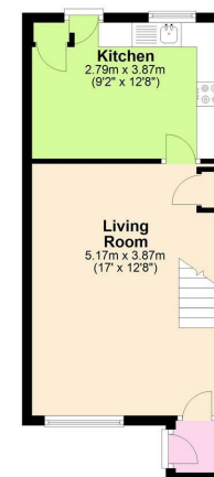
Ground Floor Approx. 32.3 sq. metres (347.6 sq. feet)
