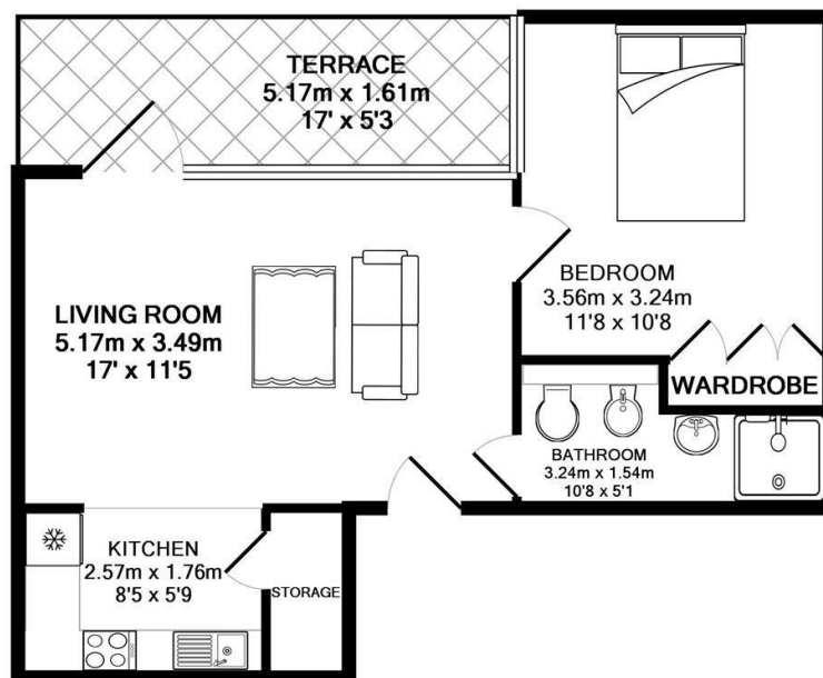
Apartment 2 - 1 bedroom Ground Floor
