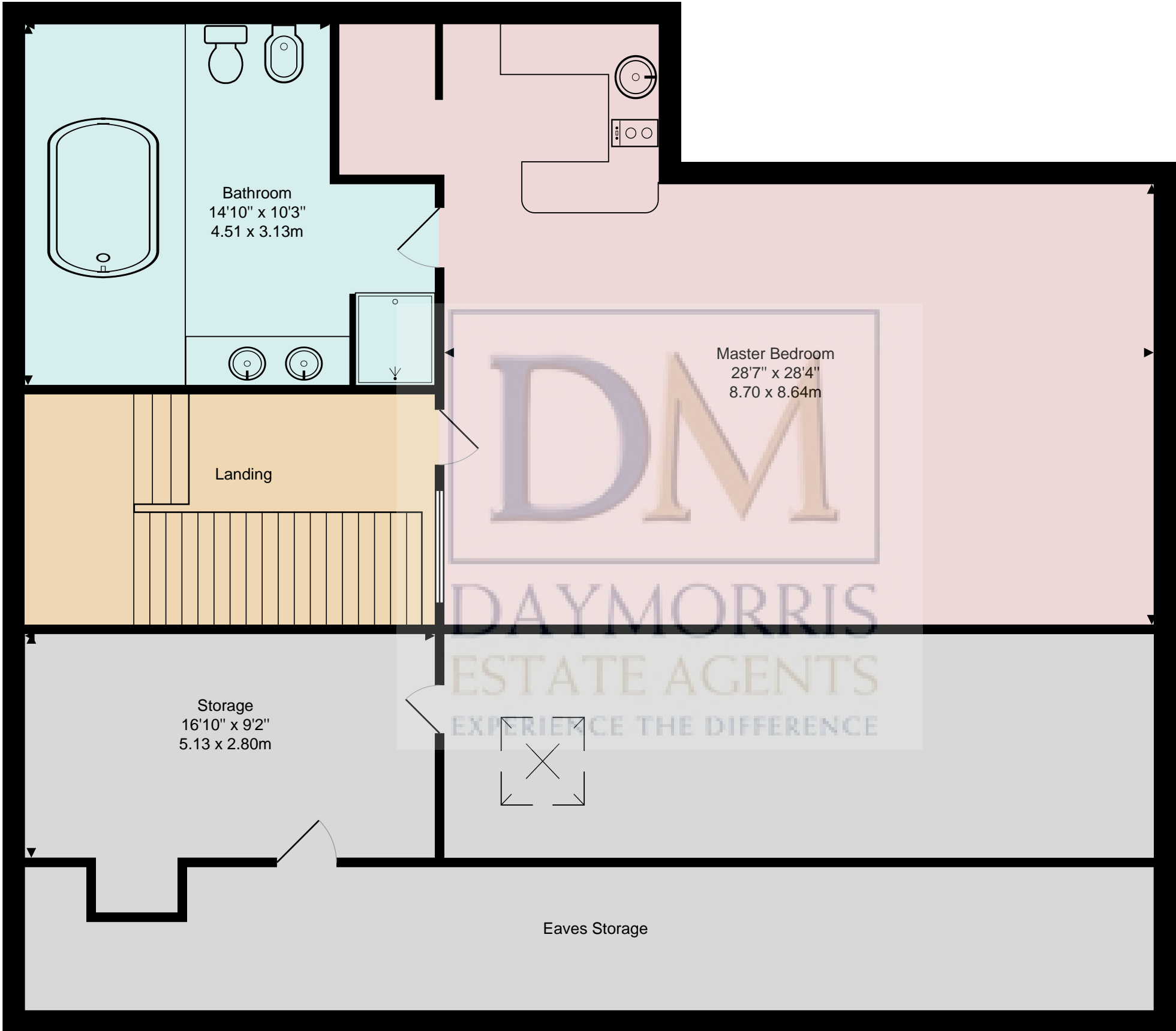
Second Floor
